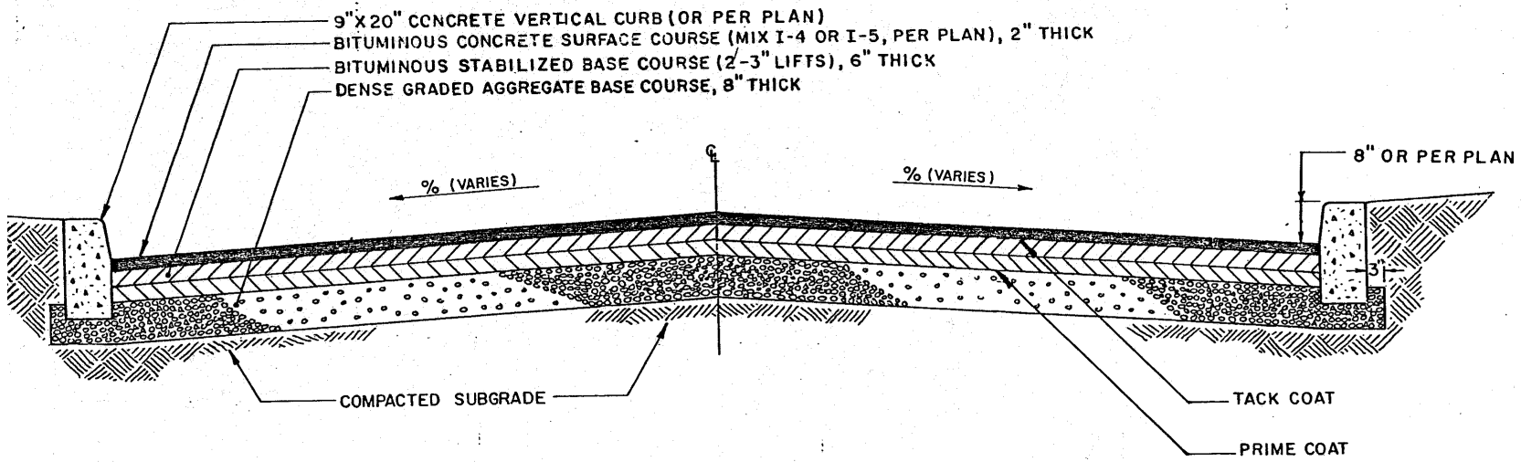
TYPICAL ROADWAY SECTION NOT TO SCALE
